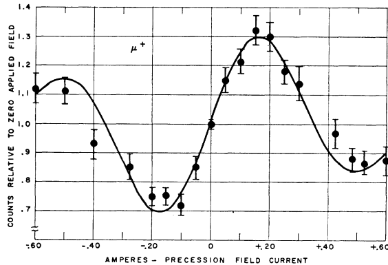
Fig. 2. Variation of gated 3-4 counting rate with magnetizing current. The solid curve is computed from an assumed electron angular distribution 1-\frac{1}{3} \cos\theta , with counter and gate-width resolution folded in.
